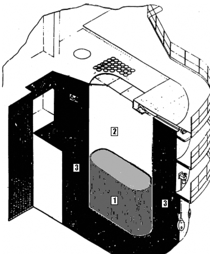
FIG. 2. The tank of the nuclear reactor after concreting. 1: grouted lower part (about 20 \text{ m}^3 ) of the reactor tank. 2: free part (about 35 \text{ m}^3 ) of the reactor tank. 3: reactor biological shielding.
